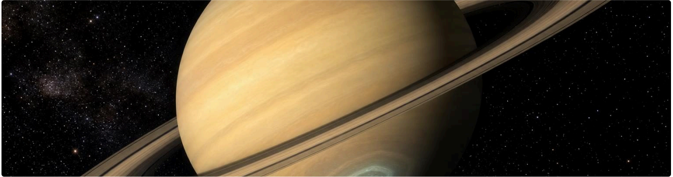
Saturn appears in space with its rings and a subtle ten-sided cloud pattern near one pole.
